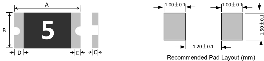
Recommended Pad Layout (mm)
