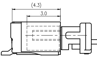
MATED CONDITION
