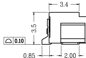
LOCK CONFIGURATION (锁扣结构)
