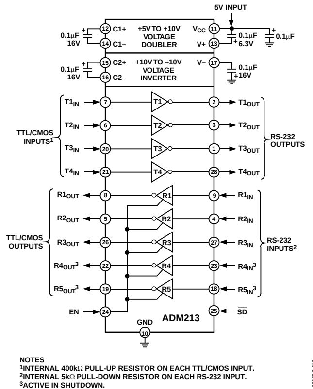
Figure 11. ADM213 Typical Operating Circuit
