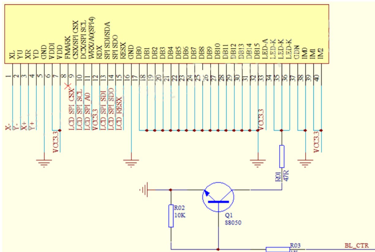
附图 6-4: 触摸屏参考应用电路 With touch version, please refer to 6-4 application circuit diagram
