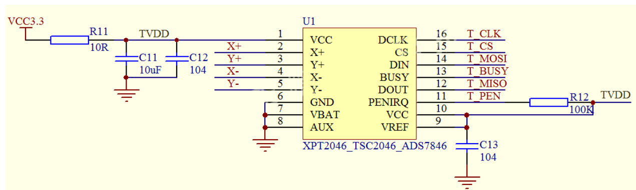
附图 6-4: 触摸屏参考应用电路 With touch version, please refer to 6-4 application circuit diagram
