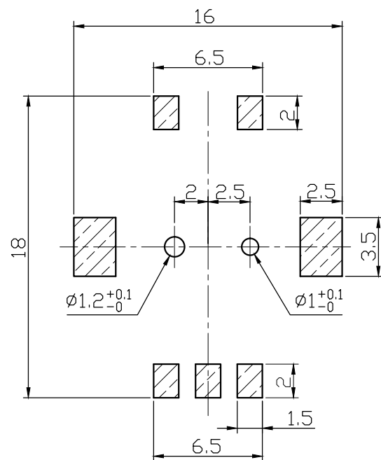
P. C. B. MOUNTING DETAIL
