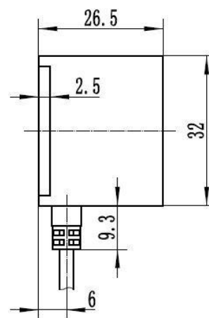
Figure 2. Top view of HPS-167U-L
