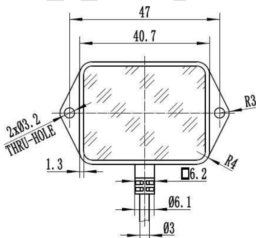
Figure 1. Front view of HPS-167U-L
