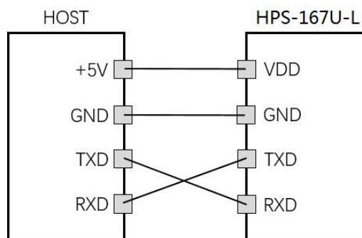
Figure. 3 Application schematic of the HPS-167U-L
