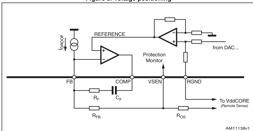
Figure 5. Voltage positioning
