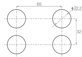
Mounting clearance
