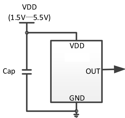
Figure 4 Typical Application
