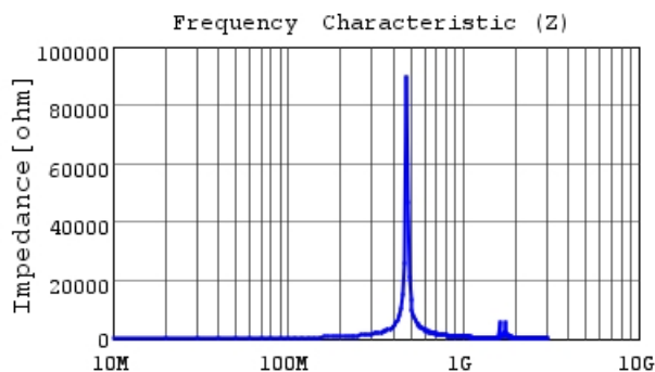
LQW2UASR56J00 |Z|
