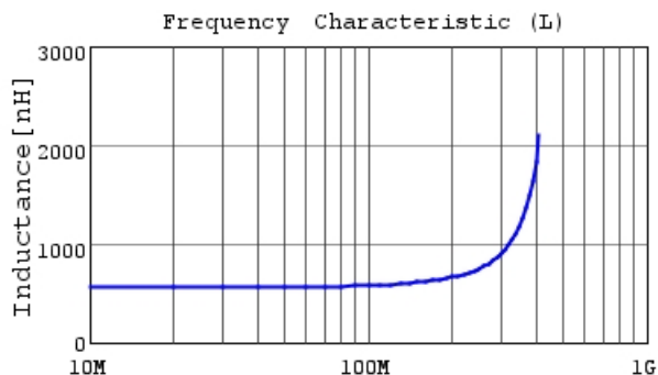
LQW2UASR56J00 L
