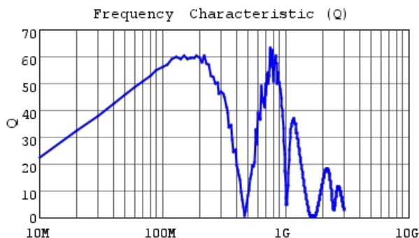
LQW2UASR56J00 Q
