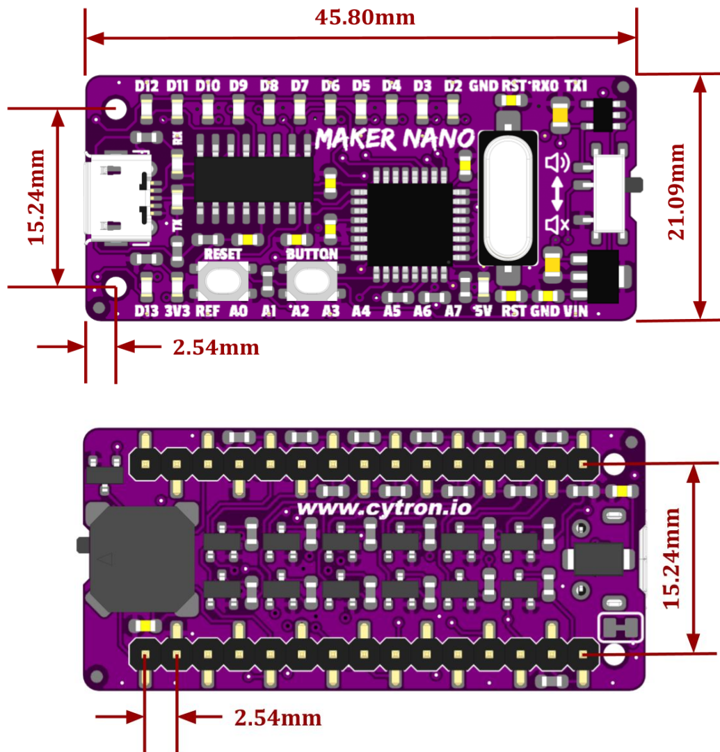
Figure 4: MAKER-NANO Dimension
