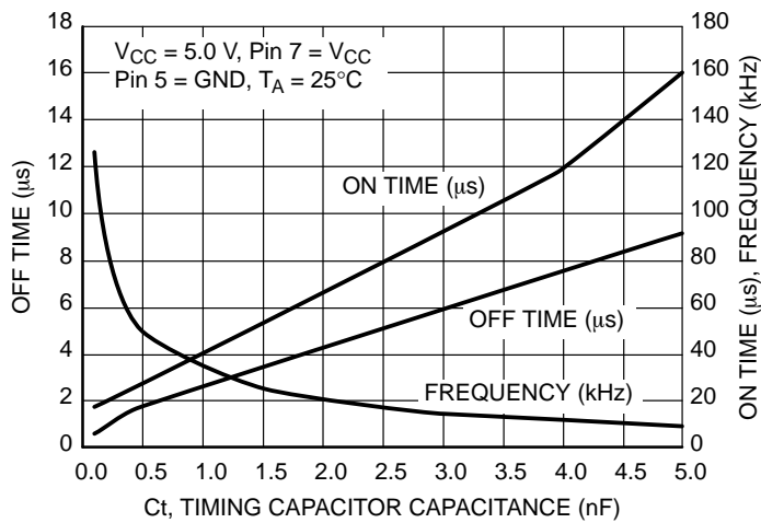
Figure 3. Oscillator Frequency
