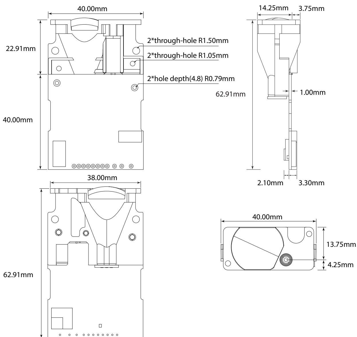
Figure 2-2 Module Structure Dimensional Diagram
