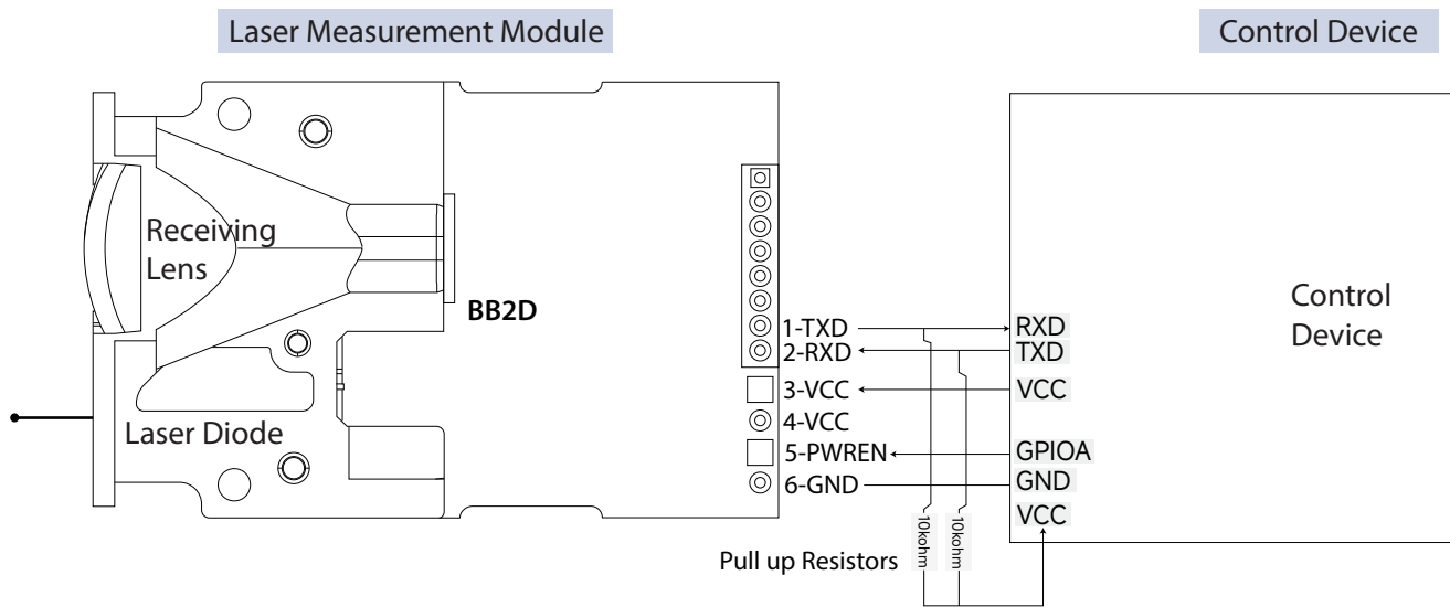
Figure 4-1 Module Pin Layout and Recommended Wiring
