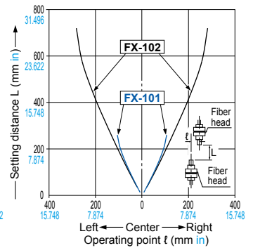
FT-A11 Thru-beam type
