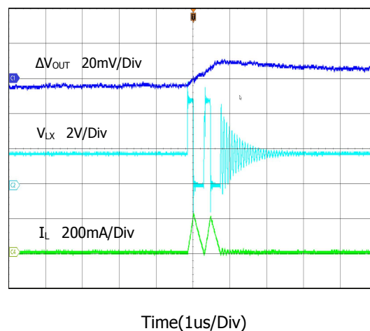
Output Ripple
