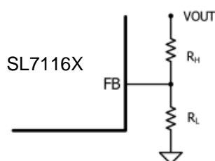
Figure 1 Feedback Network
