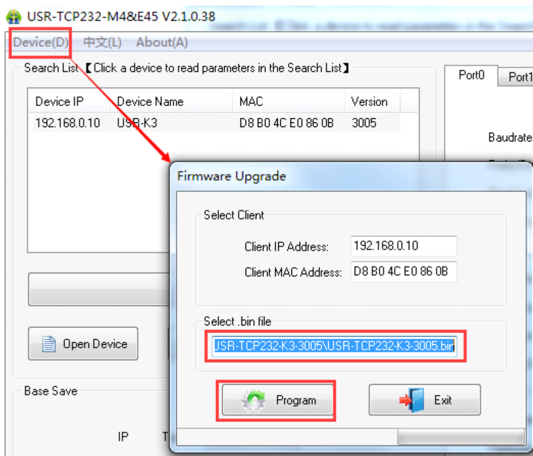
Diagram 6-13 firmware update
