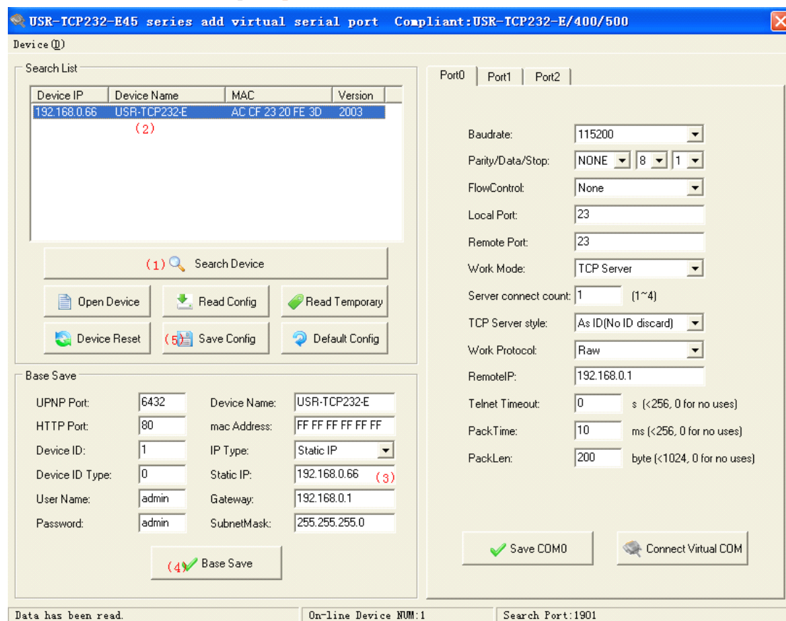
Diagram 5-1 Setup software
