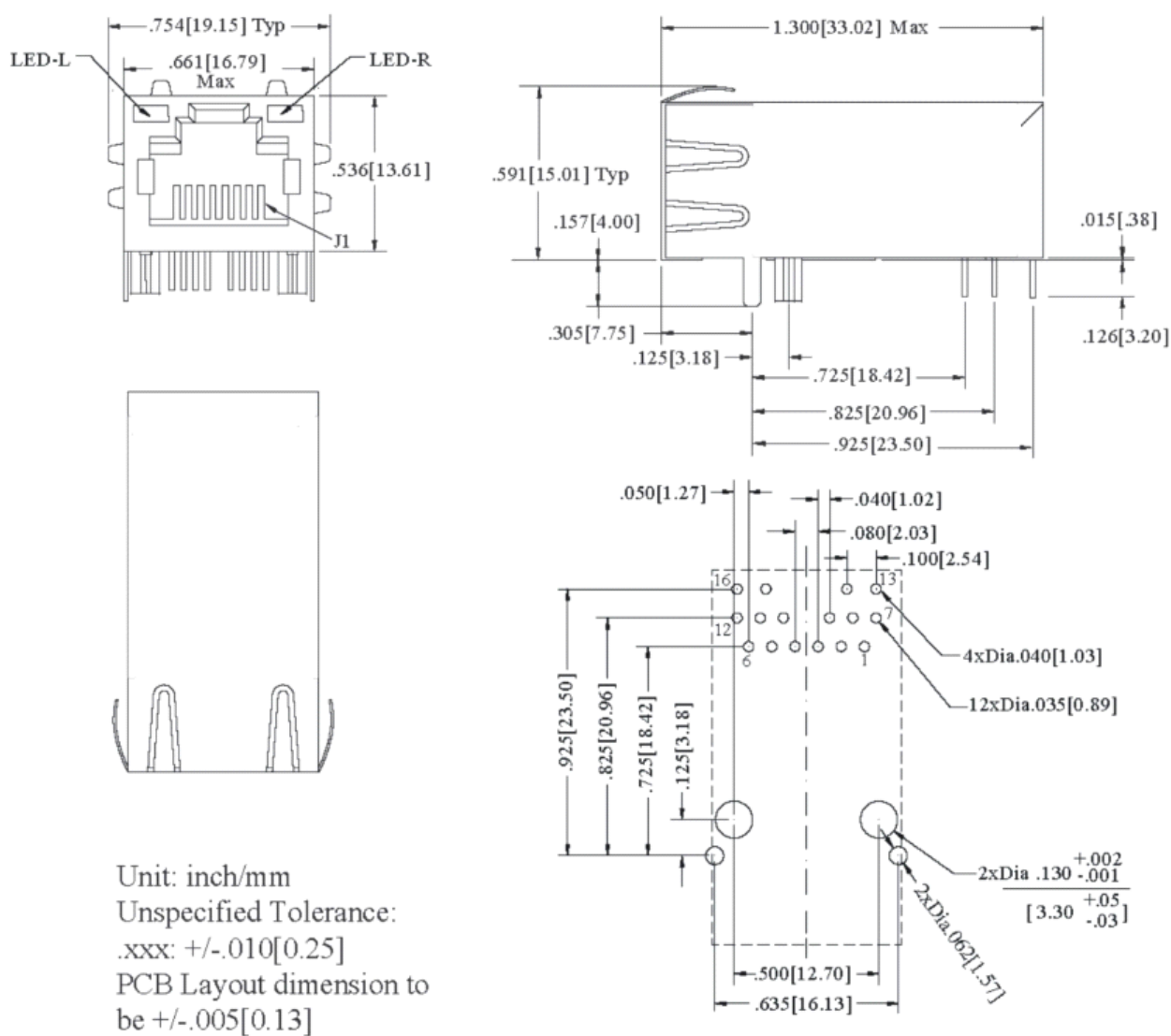
Recommended PCB Layout Component Side View
