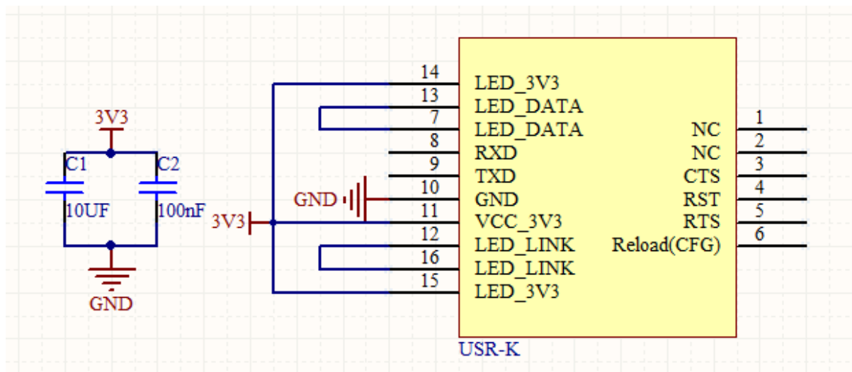
Diagram 4-5 connection diagram
