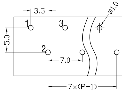
PCB layout 1
